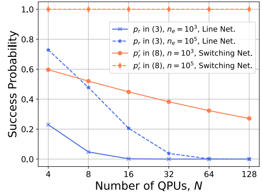
Fig. 8: Success probability vs. number of QPUs
