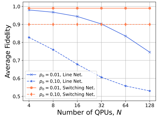
Fig. 9: Average Fidelity vs. number of QPUs
