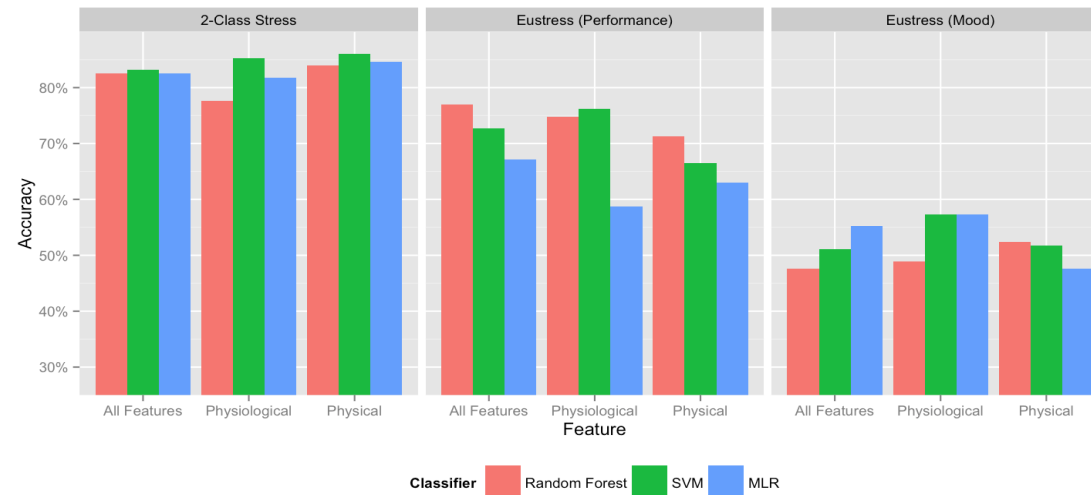
Figure 4: Classification Result
