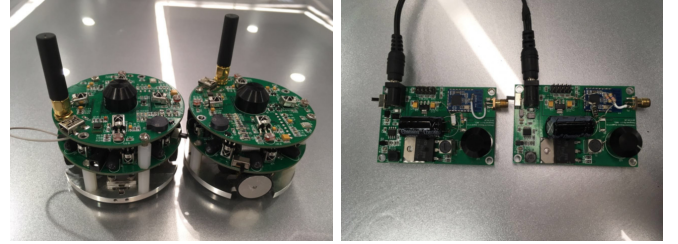
Fig. 7. The robots and the beacons
