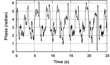
Figure 4. Raw phase values during the measurements.
