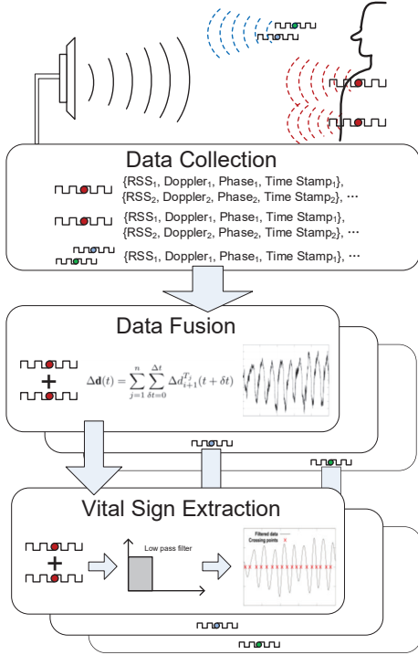
Figure 10. Illustration of TagBreathe workflow.
