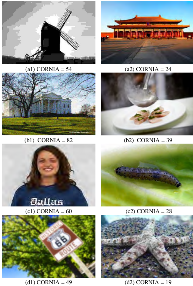
Fig. 11. Failure cases of CORNIA [12] in the P-test on the Exploration database. The left images have inferior quality compared with the right ones, but CORNIA [12] gives incorrect preference predictions.
