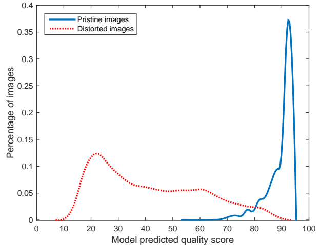
(a) WANG05 [40]
