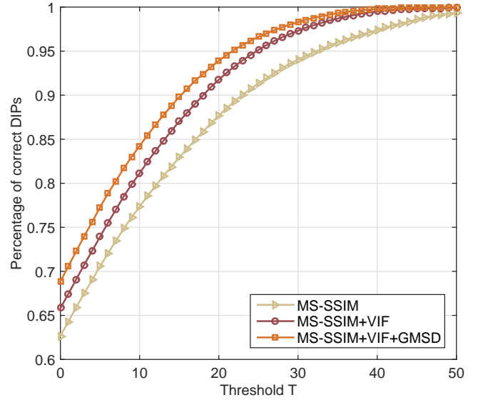
Fig. 4. The percentage of generated DIPs in the “ground truth” set on the LIVE [3] database as a function of T for different combinations of base FR-IQA models.
