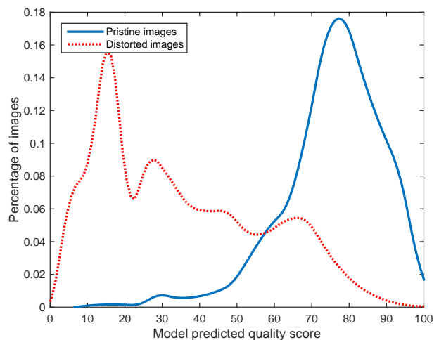
(b) DIIVINE [13]
