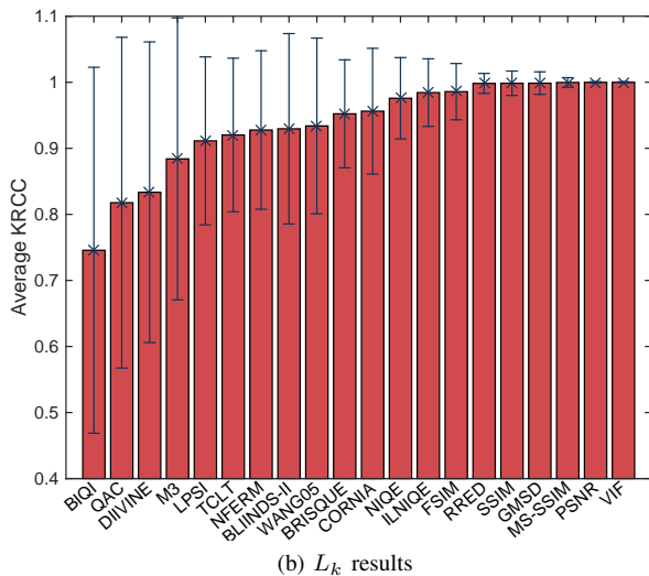
Fig. 8. L-test results of IQA models on the Exploration database.
