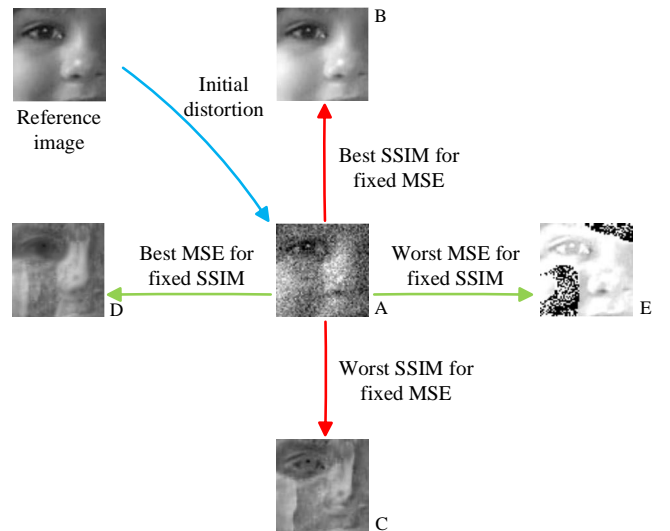
Fig. 13. Illustration of the MAD competition method [46] with synthesized image pairs.
