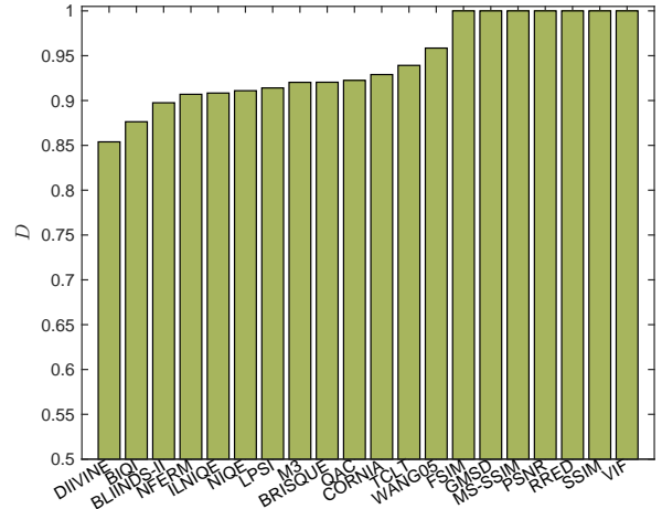
Fig. 6. D-test results of IQA models on the Exploration database.
