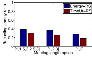
Fig. 14. Re-cooling energy ratio.
