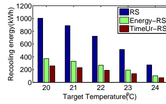
Fig. 16. Re-cooling energy as against target temperature.
