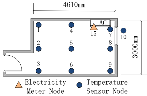
Fig. 6. Experiment Environment in the hotel room
