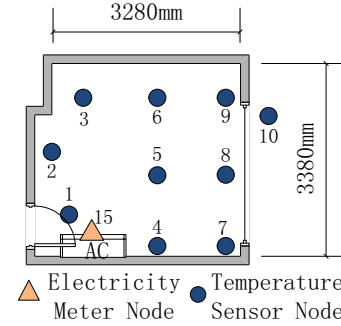
Fig. 7. Experiment Environment in the residential room
