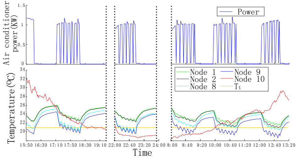
Fig. 8. Experiment Results in the hotel room
