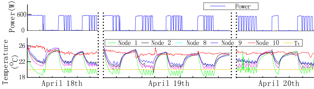
Fig. 9. Experiment Results in the residential room
