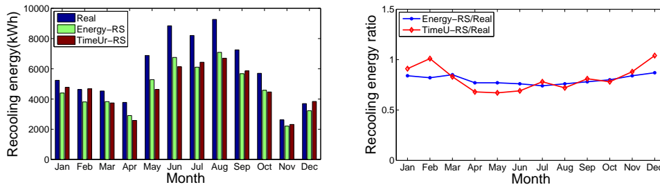
Fig. 11. Monthly re-cooling energy consumption. Fig. 12. Monthly re-cooling energy consumption ratio.
