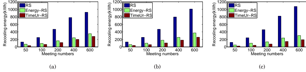
Fig. 13. Total energy expense for re-cooling the rooms as against to the number of meetings; rooms with uniform capacity. (a) meeting length: option \mathcal{O}_1 , (b) meeting length: option \mathcal{O}_2 , (c) meeting length: option \mathcal{O}_3 .
