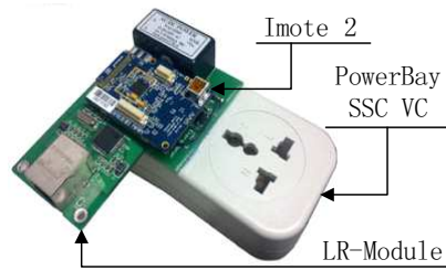
Fig. 3. An Electricity-Meter
