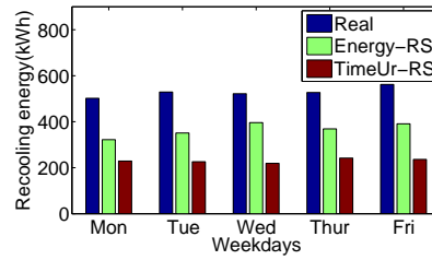
Fig. 10. Re-cooling energy in weekdays
