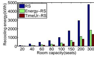
Fig. 15. Re-cooling energy as against room capacity
