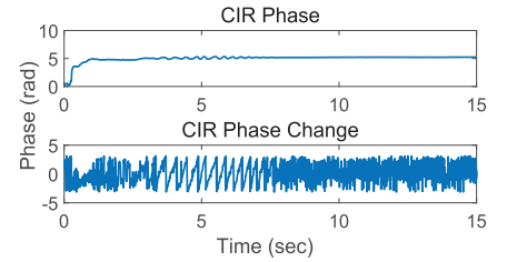
(c) CIR phase.
