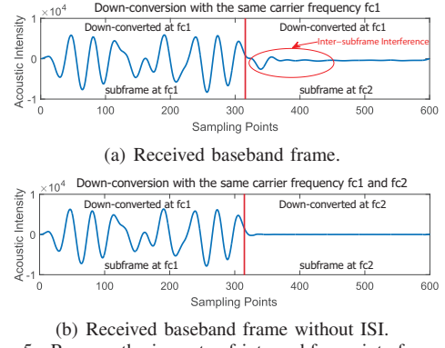
Fig. 5. Remove the impacts of inter-subframe interference.
