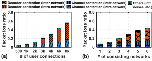
Figure 4: Decoder contention problem (a) under varying user scales of a single LoRaWAN, (b) when multiple LoRaWANs coexist (each network connects 1k users).
