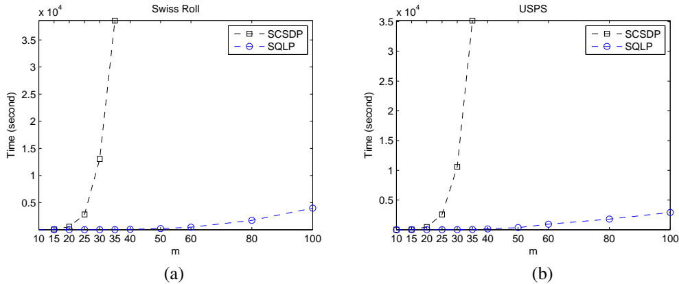
Figure 2: Curves on computational cost: Solution Time vs. Problem Scale.
