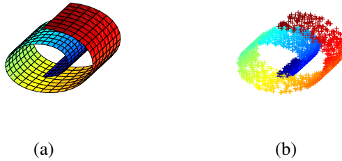
Figure 1: Swiss Roll. (a) The true manifold. (b) A set of 2000 points sampled from the manifold.
