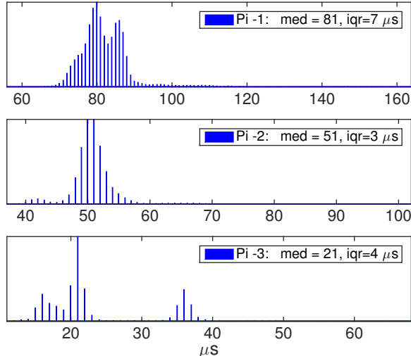
Figure 5: Kernel to user-space latency L(i) .
