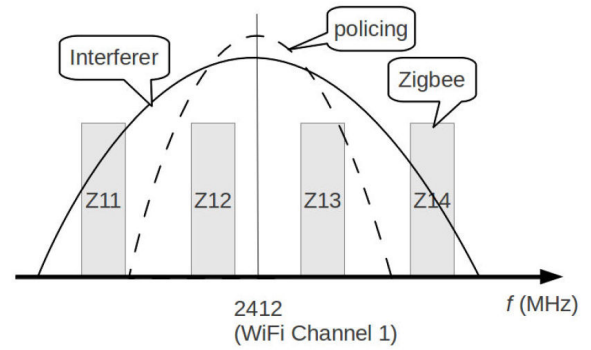
Fig. 9. PSD of WiFi interferer signal, DSSS-Nulling policing signal, and ZigBee signal
