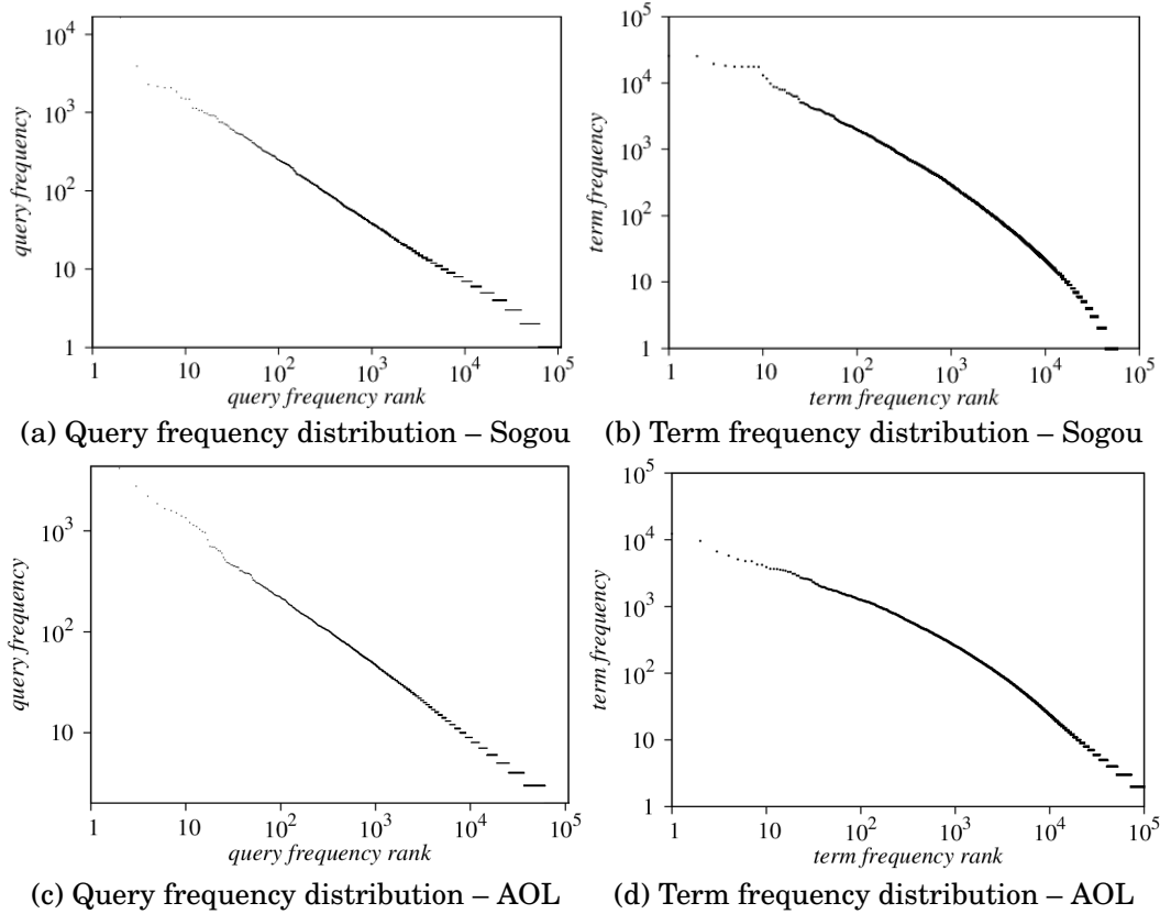
Fig. 3. Frequency distribution of our query set
