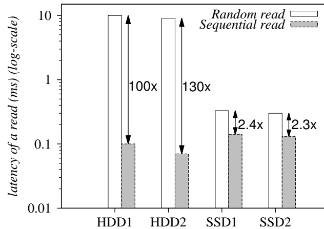
Fig. 1. Read latency on two HDDs and two SSDs. Each read fetches 4KB. The OS buffer is by-passed. Both HDDs are 7200rpm, with seek time ranging from 8ms to 10ms, maximum data transfer around 200MB/s. Both SSDs have maximum data transfer rates as 550MB/s (sequential read) and 160MB/s (random read).
