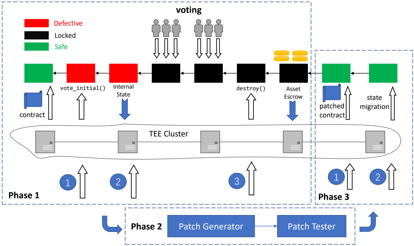
Figure 2. The workflow of SolSaviour. In Phase 1, contract stakeholders can destroy a defective contract via democratic voting. In Phase 2, a patched contract is generated and tested. In Phase 3, patched contract is deployed to replace the defective one.
