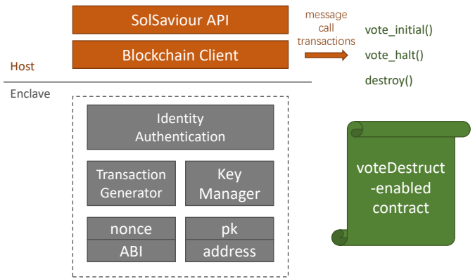
Figure 1. The architecture of SolSaviour. Contract stakeholders can invoke the TEE cluster via SolSaviour API to generate message call transactions to instruct the voteDestruct-enabled contract.
