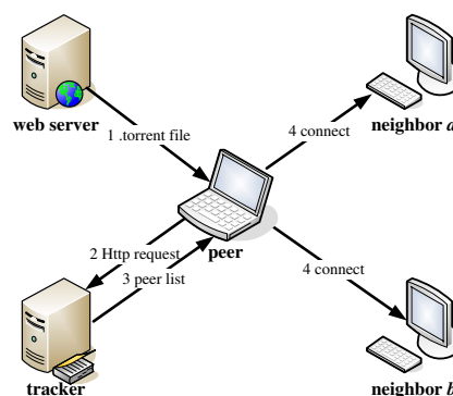
Fig. 1. The bootstrapping of BT.
