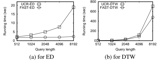
Figure 5: Response time, on RW
