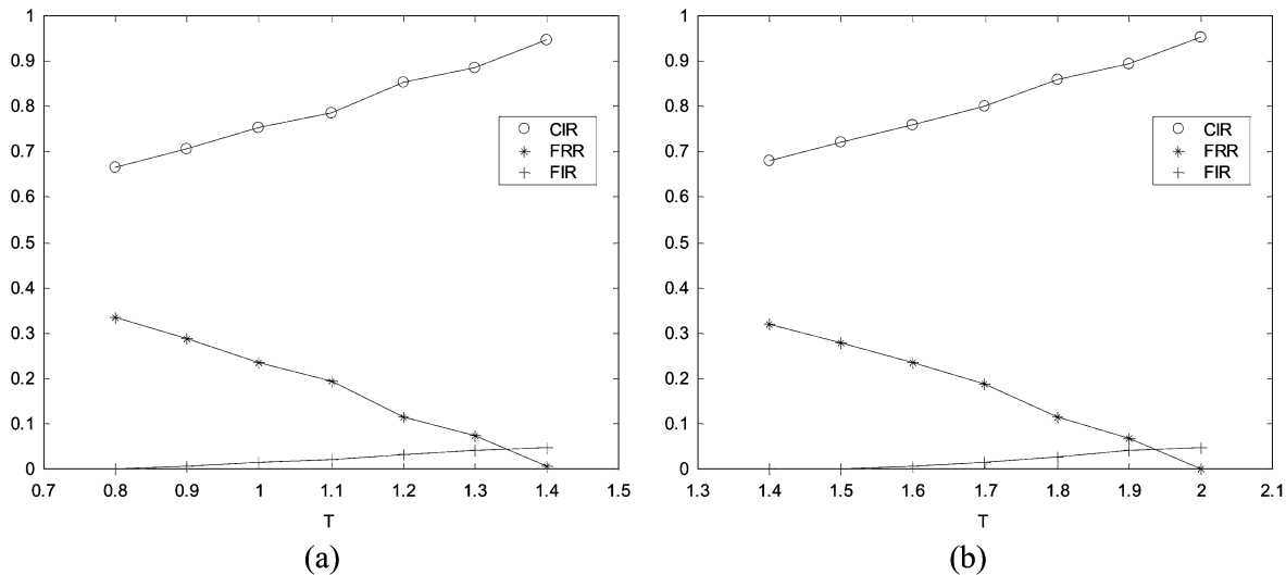
Fig. 11. Experimental results when wavelet decomposition scale is J = 2 . (a) With weight sequence \{\lambda_i\} = \{1, 0, 0, 1\} ; (b) With weight sequence \{\lambda_i\} = \{1, 0.6, 0.6, 1\} .
