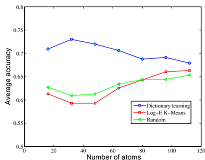
Figure 4. Classification accuracy on the Brodatz dataset
