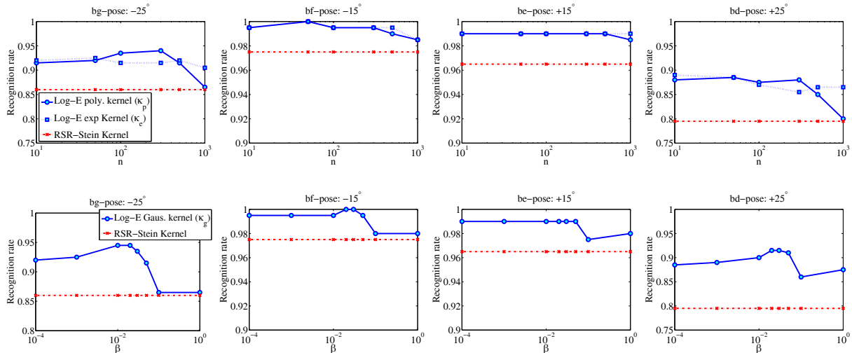
Figure 2. Classification rates on the FERET dataset. Top row: \kappa_{p_n}, \kappa_{e_n} vs. n ; bottom row: \kappa_g vs. \beta . From left to right are results on bg, bf, be, and bd, respectively. The classification rates of RSR that uses the Stein kernel [12] are shown as baseline (red dash-dotted line).
