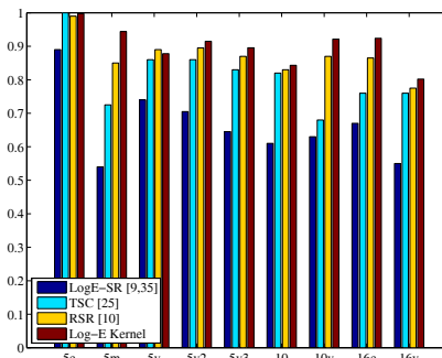
Figure 3. Classification rates on nine mosaics from the Brodatz dataset. Average rates on all nine mosaics are 0.66, 0.81, 0.87, and 0.92 for LogE-SR, TSC, RSR, and Log-E Kernel, respectively.
