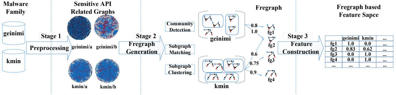
Figure 2: The overall architecture of FalDroid
