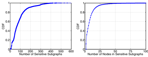
Figure 9: CDFs for number of sensitive subgraphs and number of nodes in sensitive subgraphs
