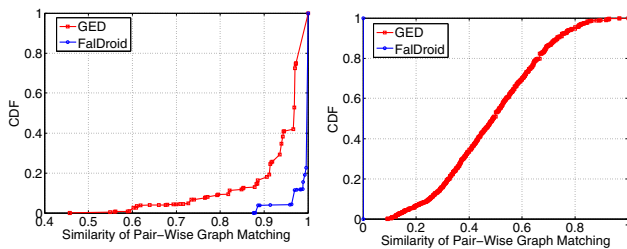
Figure 12: Effectiveness of sensitive APIs-based graph matching and GED in similar set and dissimilar set
