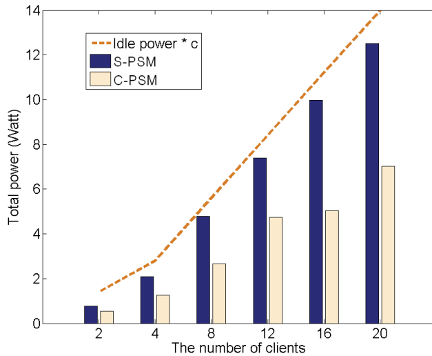
Fig. 6. Total power verses c under the EXP distribution with \delta_j = 10 + 5j(\text{ms}), j = 1, \dots, c .
