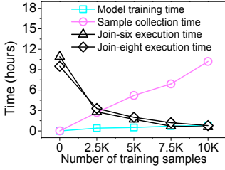
Fig. 20. Training and execution time with varying number of samples.
