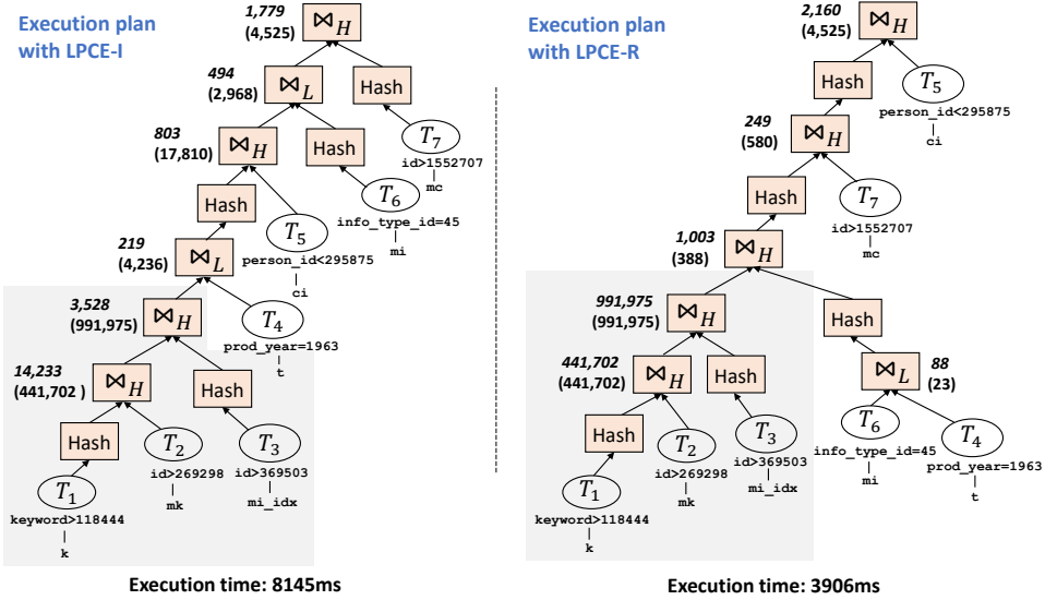
Fig. 17. An example of query re-optimization. Upright number for real cardinality and italic number for estimated value. Shaded area indicates executed sub-plan.
