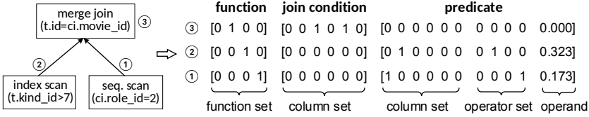
Fig. 6. Example for feature encoding.
