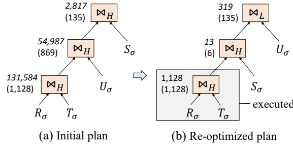
Fig. 3. Query re-optimization example, upright number for real cardinality and italic number for estimated value. \bowtie_L indicates nested loop join and \bowtie_H is hash join.
