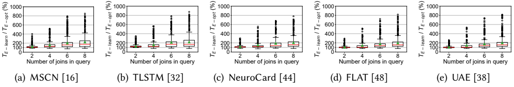
Fig. 2. Effect of estimation error on execution time. T_{E-learn} and T_{E-opt} are the query execution time when using the estimated and actual cardinalities for plan search. T_{E-learn}/T_{E-opt} increases with more joins as errors in Figure 1 become larger.
