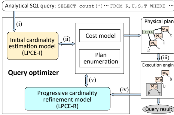
Fig. 4. End-to-end query execution with LPCE.
