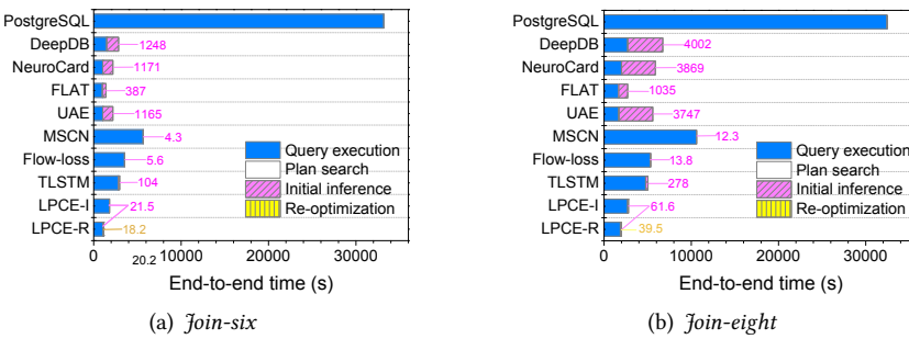
Fig. 12. Decomposition of end-to-end query execution time. The colored numbers indicate the time spent on model inference (in pink) and re-optimization (in yellow).
