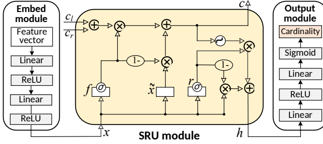
Fig. 7. The structure of the SRU-based model in LPCE-I.
