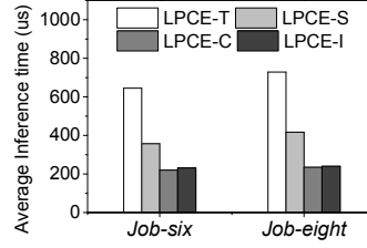
Fig. 21. Average model inference time for one cardinality.
