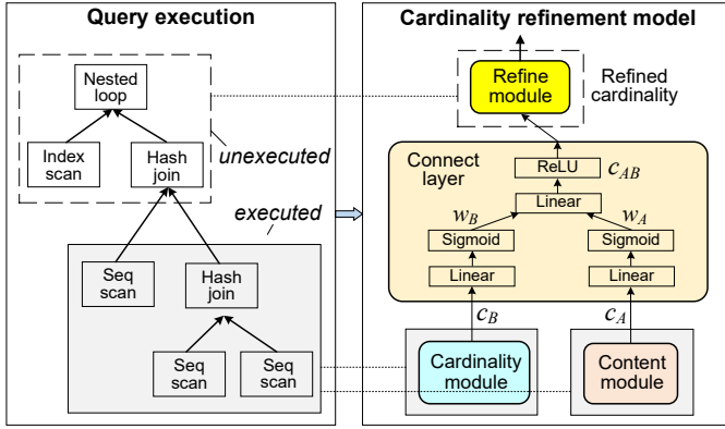
Fig. 9. An overview of LPCE-R for estimation refinement.
