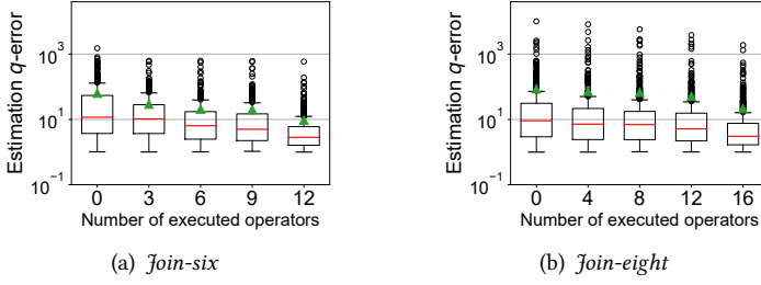
Fig. 16. The change of the mean q -error for LPCE-R in the query execution process.
