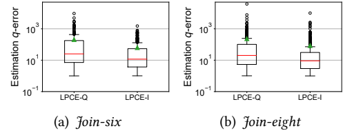
Fig. 23. Effect of node wise loss function on accuracy.
