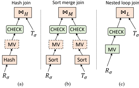
Fig. 11. Modifications of the join operators to support query re-optimization, color brown indicates the original operator logic in PostgreSQL while color green indicate our modifications. ‘MV’ means tuple materialization.
