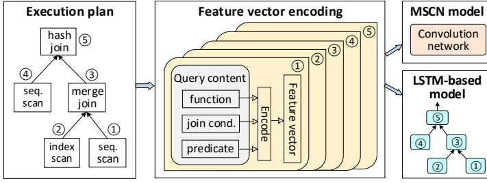
Fig. 5. Workflow of learning-based estimation model.
