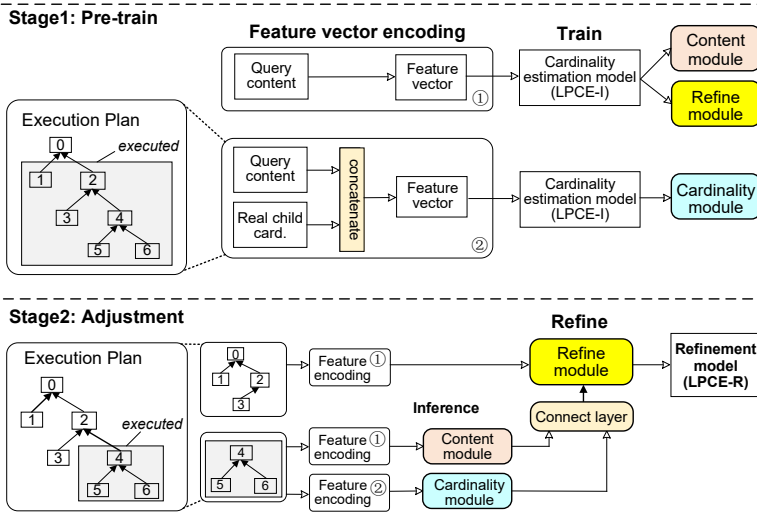
Fig. 10. The training workflow of LPCE-R.
