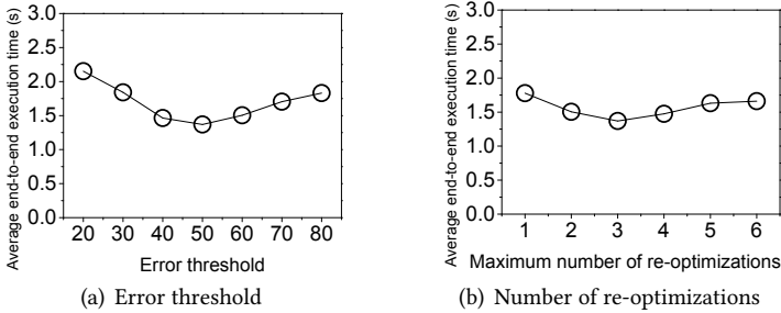
Fig. 18. Influences of the re-optimization parameters.
