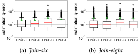
Fig. 22. Effect of SRU and distillation on accuracy.
