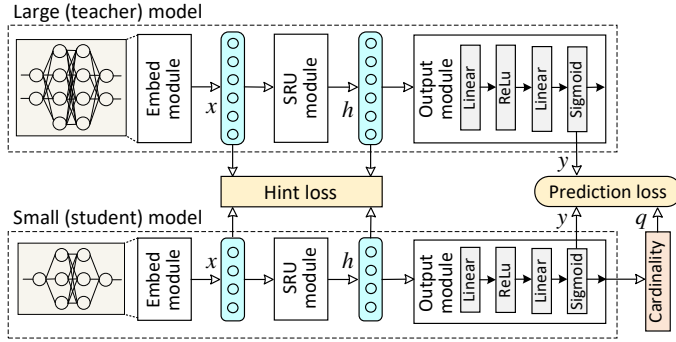
Fig. 8. Model compression via knowledge distillation.
