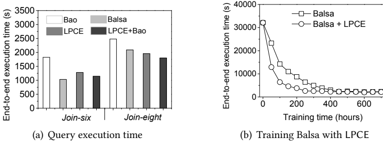
Fig. 19. Comparing and combining LPCE with two learned optimizers.
