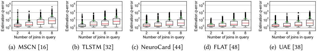
Fig. 1. Estimation error for queries with different number of joins. Red line and green triangle indicate median and mean, black rectangle shows 25th and 75th percentile, the black lines indicate 5th and 95th percentile, and circles are extreme errors.
